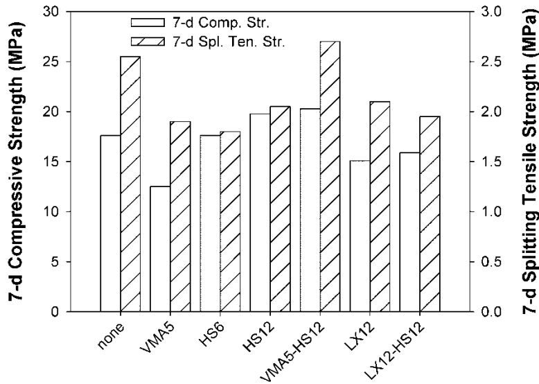
Figure 26. Effect of admixtures on strength (B24[50,35,15]-S10-CS1.5-w/c0.29)
