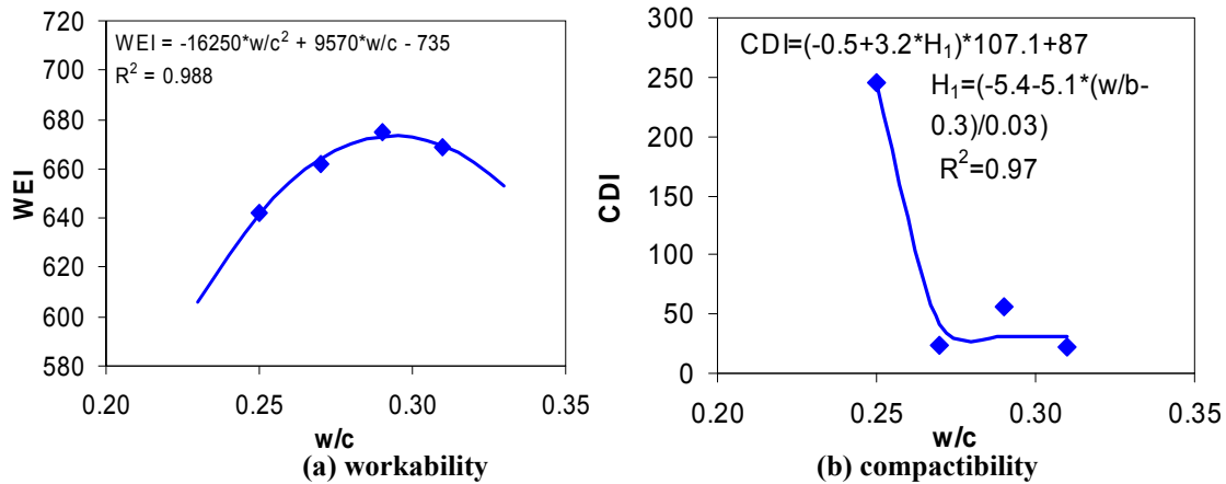
Figure 19. Effect of w/c on workability and compactibility
